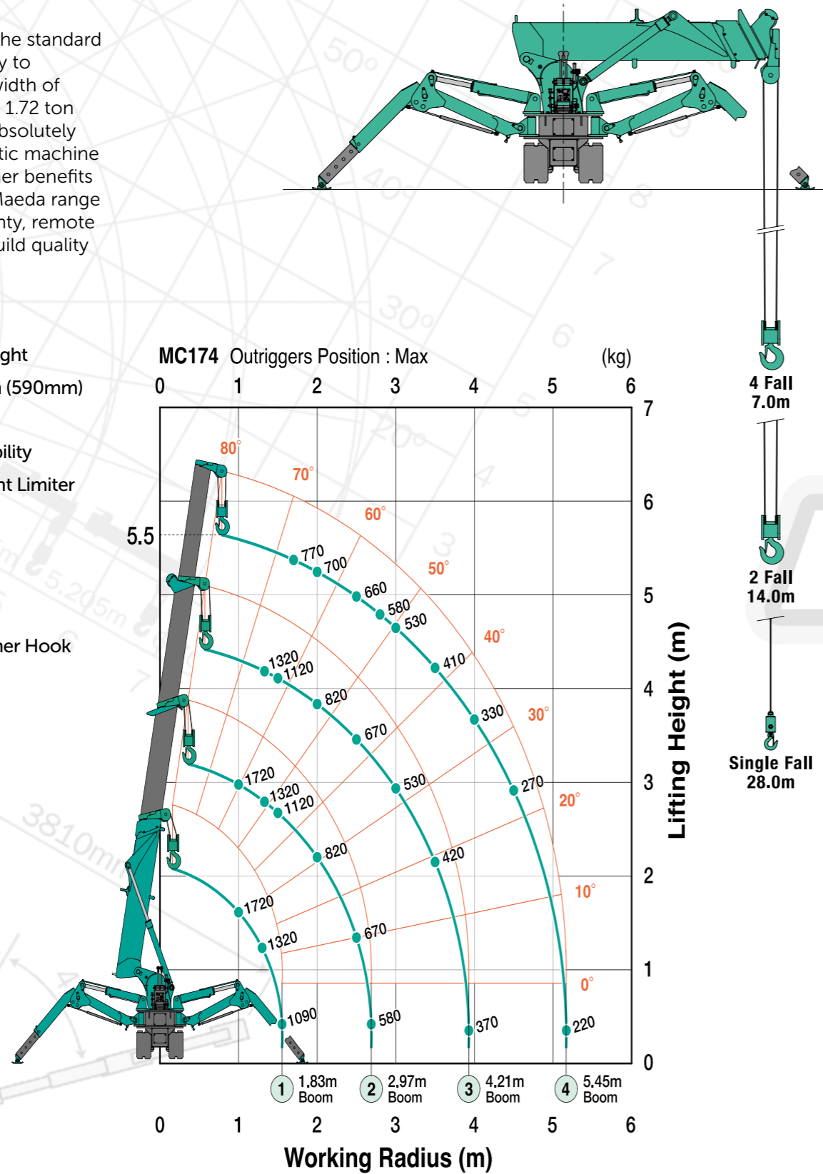
This working range chart shows total rated load including boom deflection.
